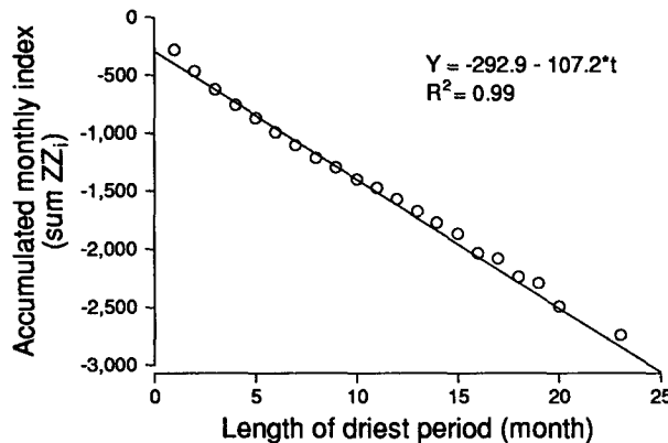
FIG. 2. The accumulated moisture anomaly index ( \sum ZZ_i ) during the driest periods of various lengths.
